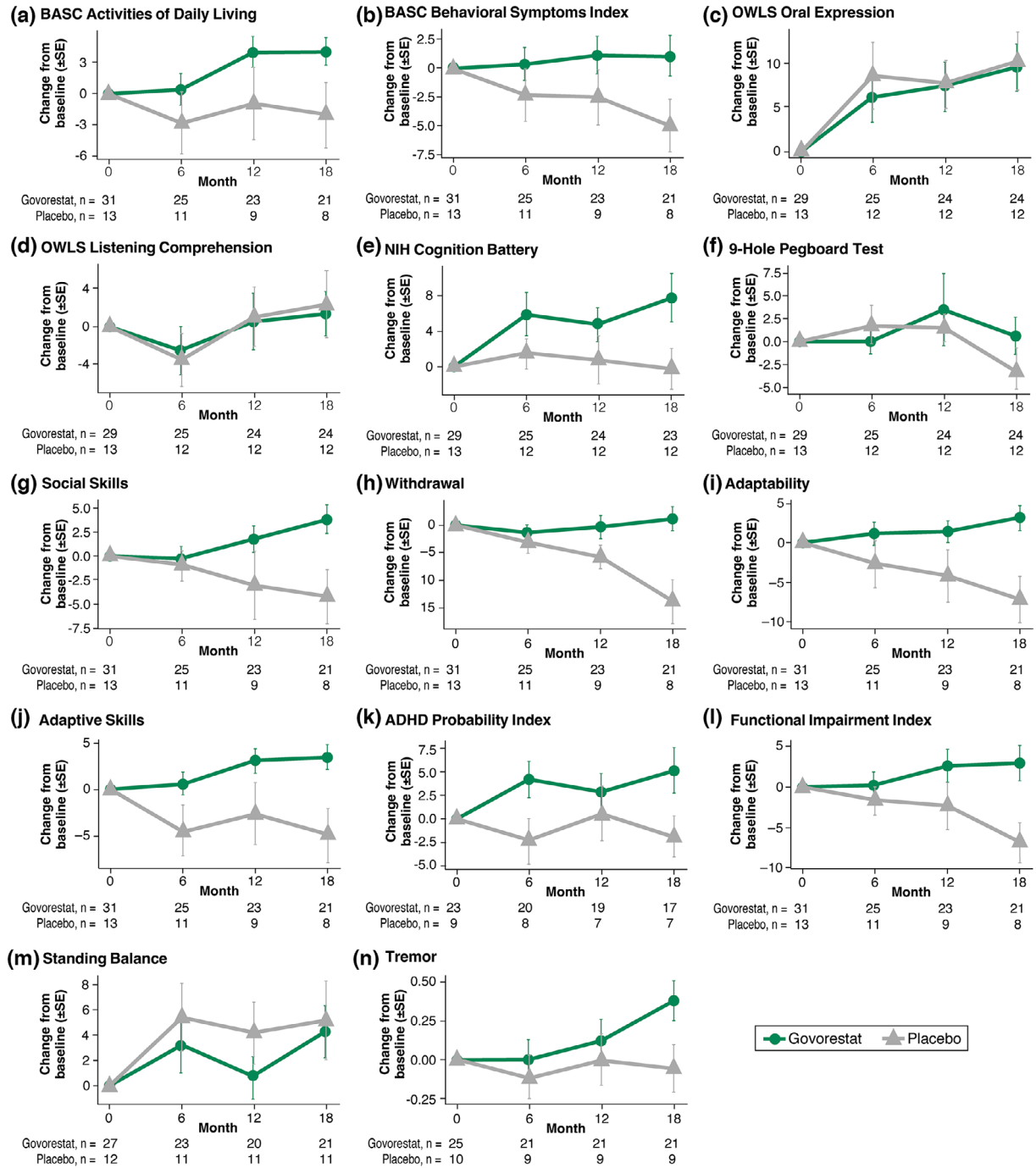
Figure 3. Mean change from baseline to 6, 12, and 18 months for the govorestat and placebo treatment groups on age-standardized tests. (a) Behavior Assessment System for Children Activities of Daily Living (BASC-ADL). (b) Behavior Assessment System for Children Behavioral Symptoms Index (BASC-BSI). (c) Oral and Written Language Scales-Oral Expression (OWLS-OE). (d) Oral and Written Language Scales-Listening Comprehension (OWLS-LC). (e) National Institute of Health Cognition Battery (NIH-CB). (f) 9-Hole-Pegboard Test (9HPT). (g) BASC social skills. (h) BASC withdrawal. (i) BASC adaptability. (j) BASC adaptive skills. (k) BASC attention deficit hyperactivity Disorder (ADHD) probability index. (l) BASC functional impairment index. (m) NIH standing balance test. (n) Tremor (not age standardized). For all graphs, error bars show standard error (SE).
